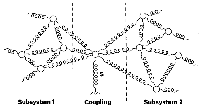
FIG. 1. Two finite-degree-of-freedom mechanical systems are coupled together via a single extra degree of freedom, corresponding to movement in one direction only of the mass m which is restrained by the spring S . For simplicity only the elastic structures are shown: dashpots are omitted. The coupling can be made weak in a number of ways, the one we discuss first being to make the spring S very strong compared with the other springs in the system. The systems can be completely decoupled by letting S become infinitely stiff. As an example of realistic coupled subsystems which can be represented in discrete form like this, consider two sections of cylinder separated by a rib; if in the frequency range of interest the ring of rib had just one resonance, its motion could be adequately described by a single degree of freedom representing the corresponding mode shape. We would certainly expect that such a resonance in the coupling would have a significant effect on power flow between the subsystems.
