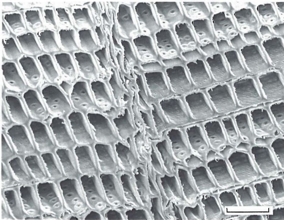
Fig. 1. Transverse section of modern air-dried spruce. Scale bar = 100 \mu\text{m} .
