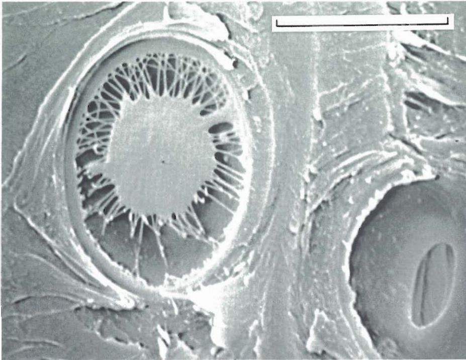
Fig. 6. Sample from a violin by Testore, c. 1700. Scale bar = 10 \mu\text{m} .
