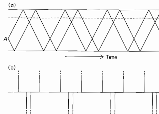
Figure 1. (a) Space-time diagram of impulses travelling on a stretched string; (b) time series seen by the observer represented by the dashed line in (a).
